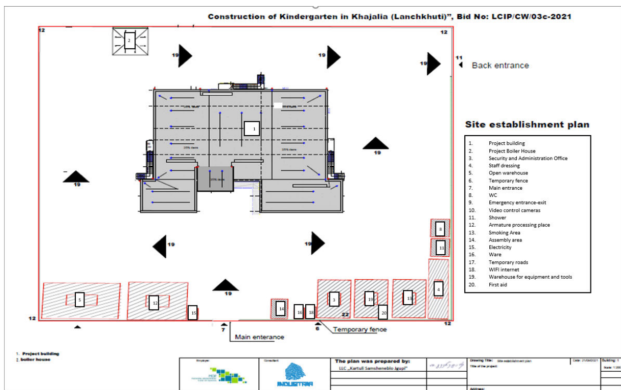
Figure 6 Construction site organization scheme
